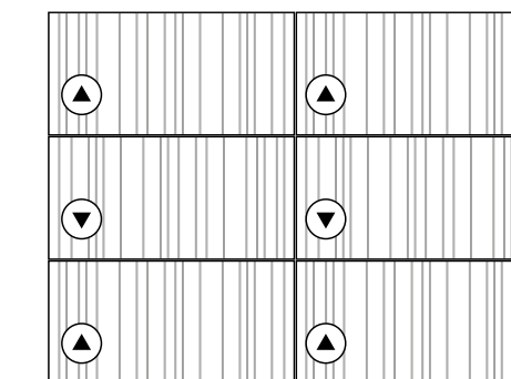
LAYING PATTERN 2
